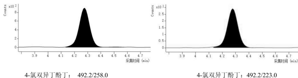
图 C.1 4-氯双异丁酚丁提取离子色谱图 (10 ng/mL)
